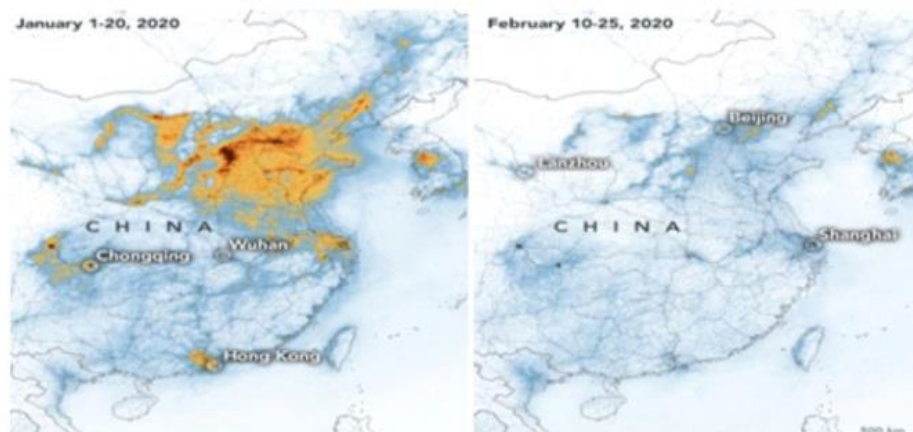
Fig. 1. TROPOMI data shows the NO 2 levels in China in the beginning of 2020[2]
